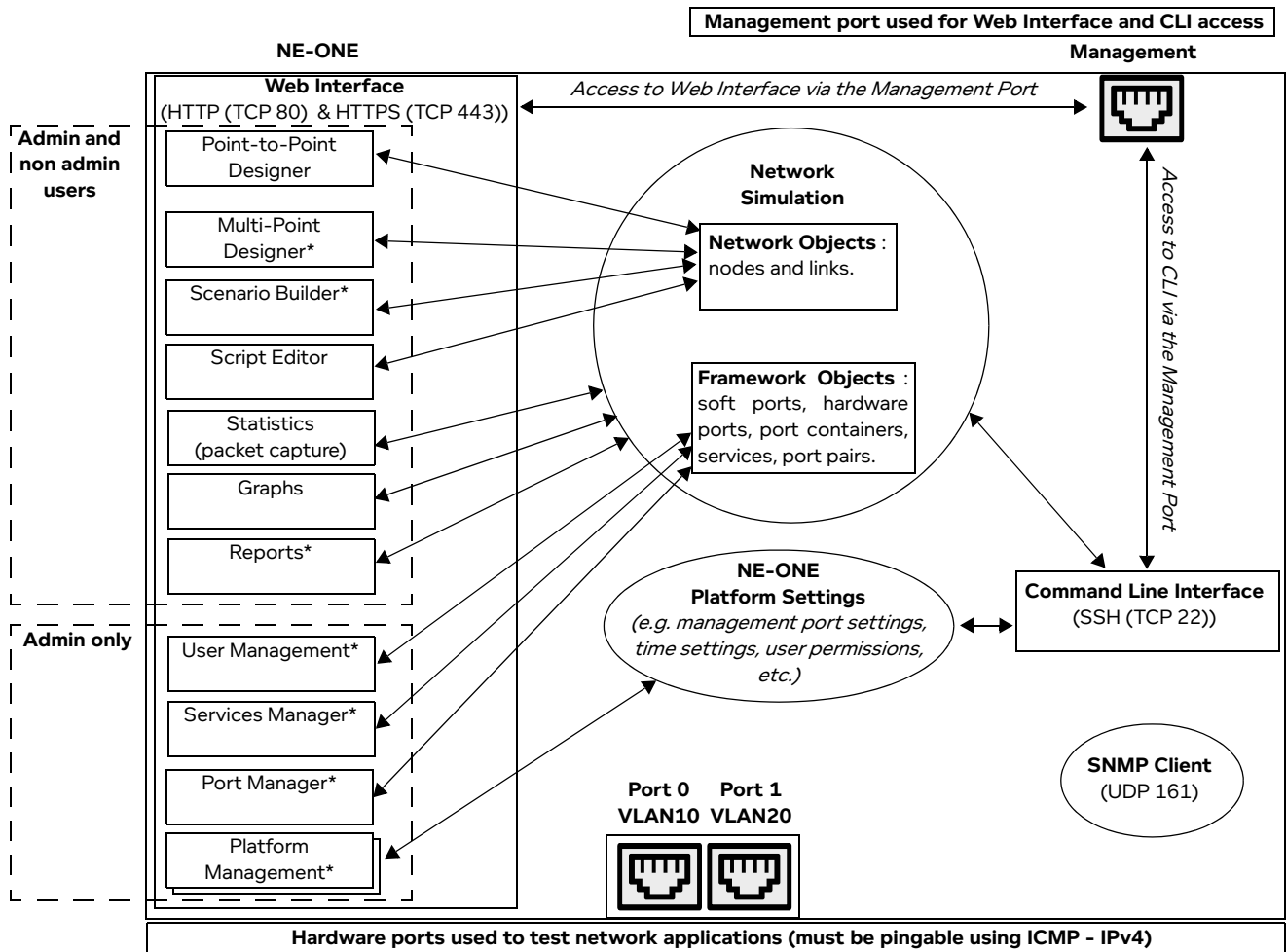
ILLUSTRATION 2 - HIGH-LEVEL FUNCTIONAL OVERVIEW OF THE NE-ONE
